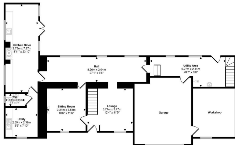
Ground Floor Approx 137 sq m / 1480 sq ft
